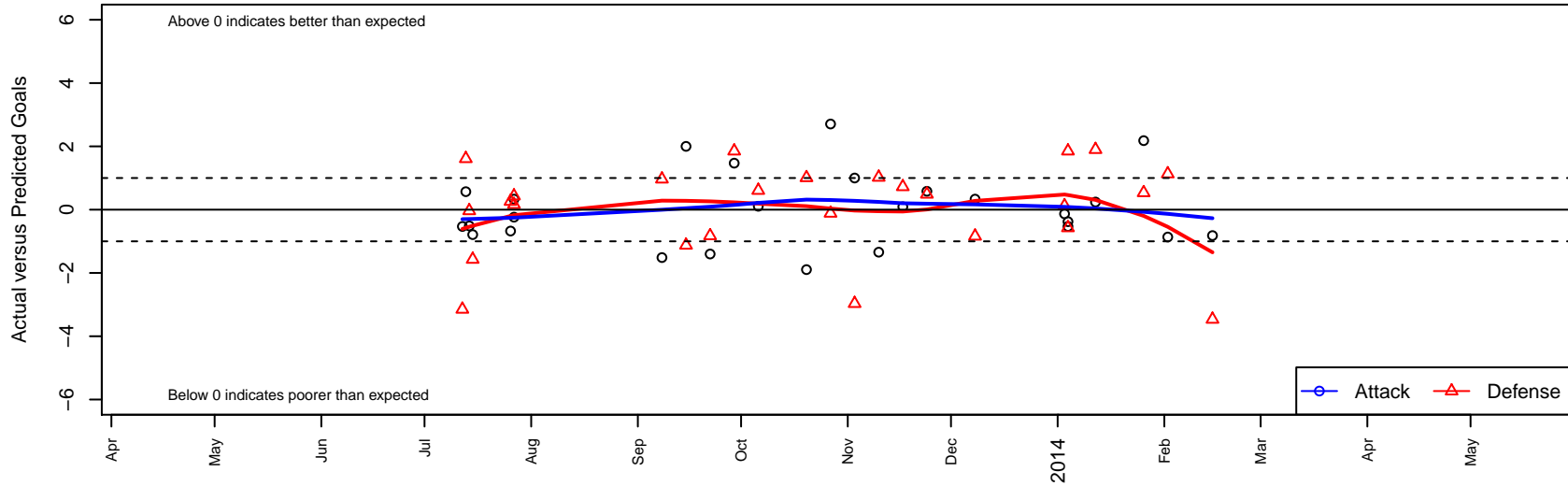
Slammers Orange B95 Dots are actual minus expected GF (blue circles) and GA (red triangles). Blue line is smoothed change in attack strength. Red is smoothed change in defense strength.
